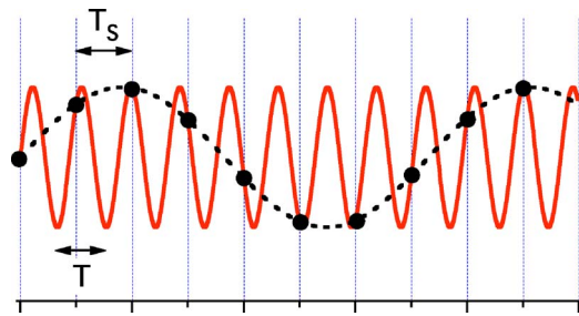
FIG. 22. (Color in online edition) Aliasing of a high-frequency signal (solid curve, with period T ) produced by sampling with a period T_s that is greater than the Nyquist criterion. The apparent measured points (large dots) are interpreted as coming from a much lower frequency signal (dashed curve).
