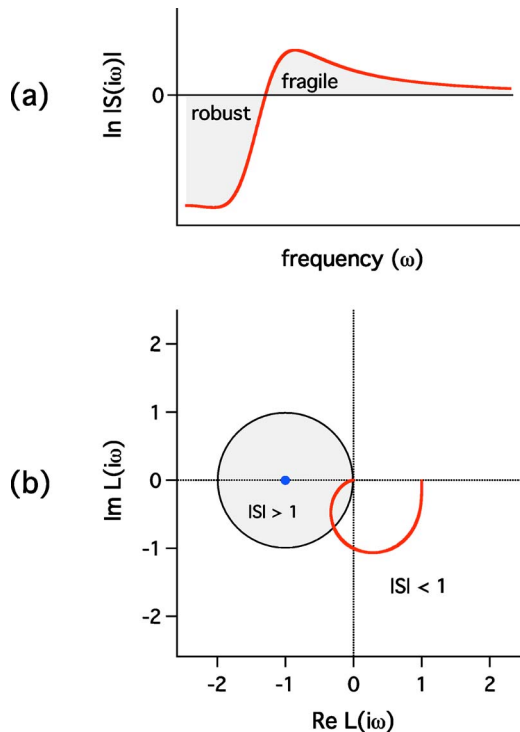
FIG. 28. (Color in online edition) Constraints on the sensitivity function S=1/(1+L) . (a) Logarithm of the sensitivity function \ln|S(i\omega)| for a second-order system with proportional gain. The negative area where control is “robust” is just balanced by the positive area, where control is “fragile.” Note that the slow decay (here, \ln|S| \sim \omega^{-2} at large frequencies) implies that a significant part of the positive area is off the plot. (b) Nyquist plot of the same system. Note that when the plot enters the shaded circle of radius 1, centered on -1 , we have |S| > 1 .
