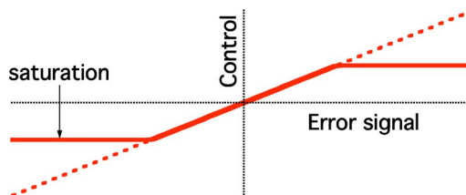
FIG. 30. (Color in online edition) Saturation of proportional gain. Thin dashed line is the proportional gain with no saturation. Thick lines show saturation. There is, in general, no reason for saturation to be symmetric about zero, as depicted here.
