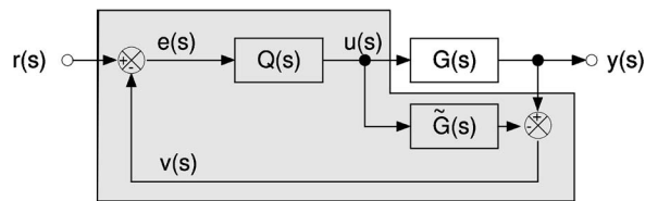
FIG. 25. Block diagram of an IMC controller. Shaded area is implemented either in a computer program or in control electronics.
